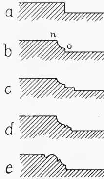
FIG. 358. CROSS-SECTIONS OF MOULDINGS USED IN CARVING TRACERY.
